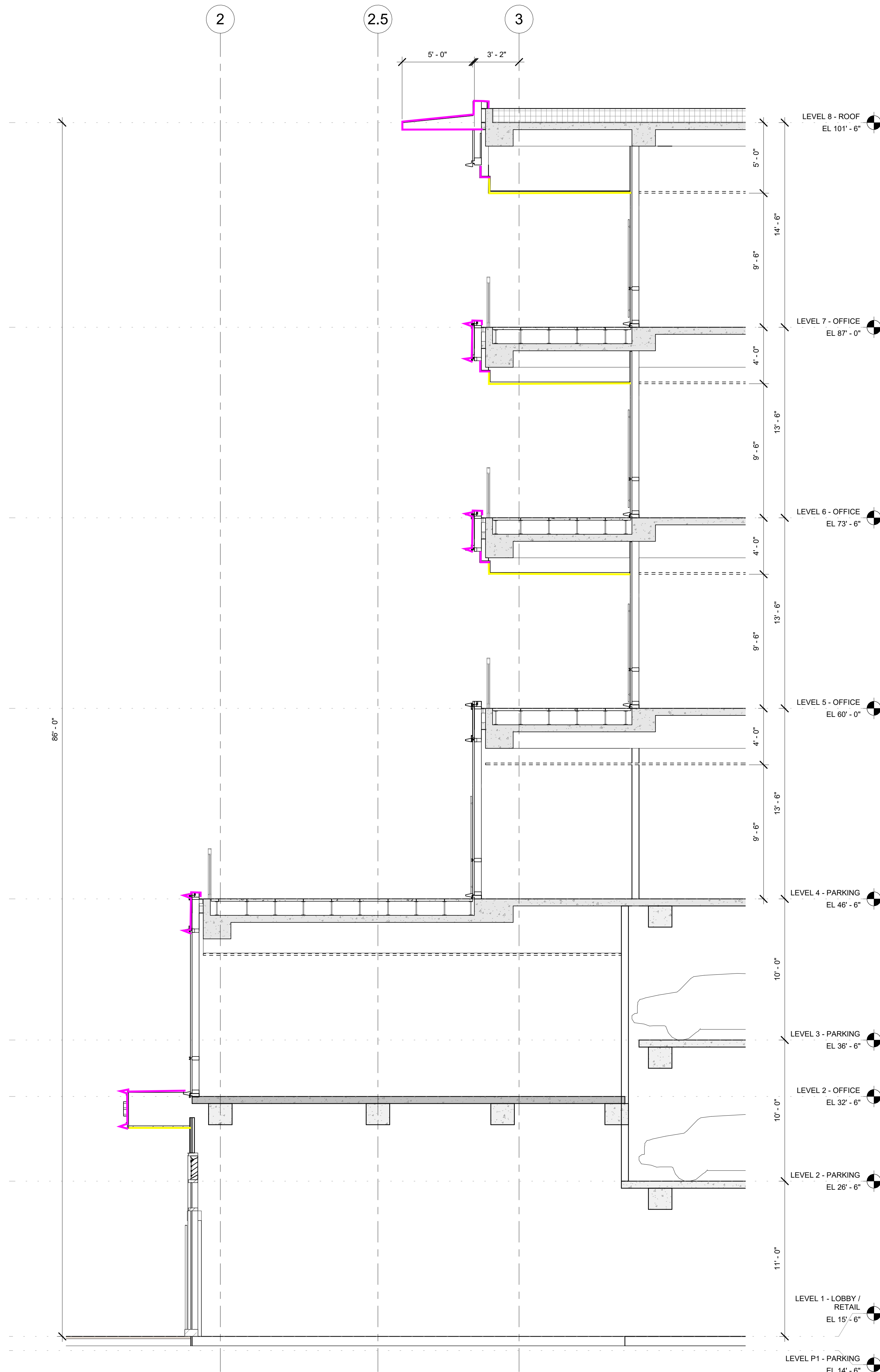
2 WALL SECTION 1/4" = 1'-0"
